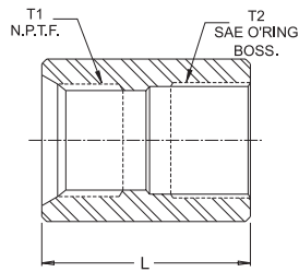
SAE/NPT COUPLING
