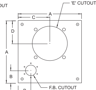
Cover with Filler Breather Cutout and 182TC/256TC Adapter Cutout (Adapter Style 6) Part Number 99943
