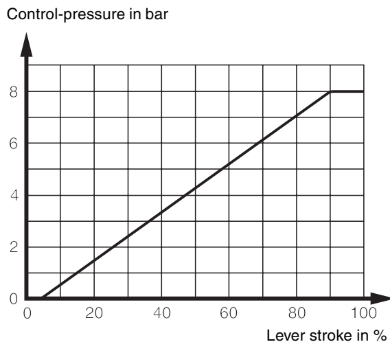
Diagram showing control-pressure characteristic of the VP04-valve. Valid for 8 - 10 bar supply pressure. If lower the curve will level out at obtained supply pressure.
