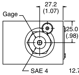
End View
