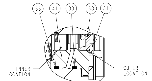
SINGLE SHAFT SEAL ASSEMBLY P2-060-0210-01□ SECTION A-A SCALE 1:1
