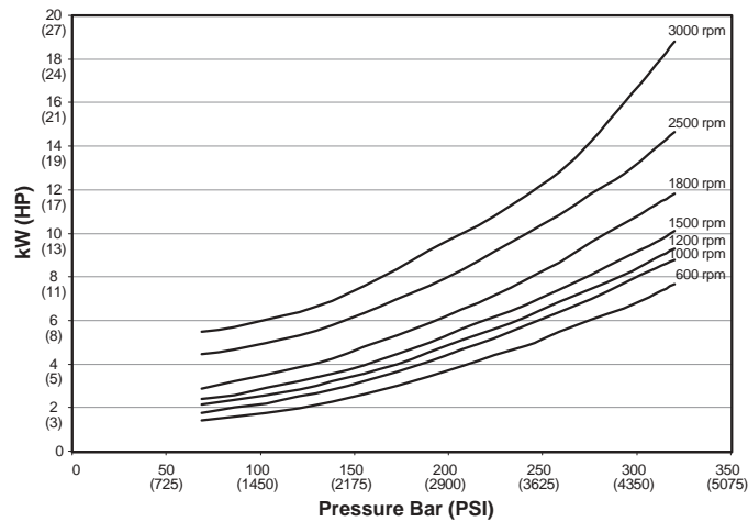
P3075 Input Power - Zero Stroke
