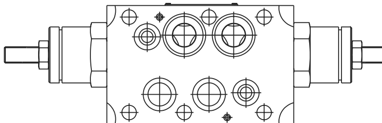
Bottom View
