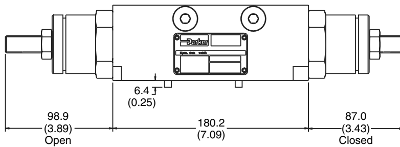
Face View
