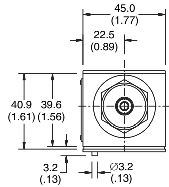
End View
