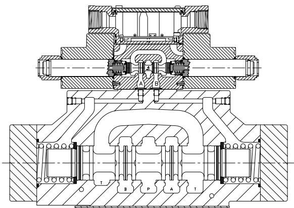
D81VW Solenoid Operated Conduit Box Style
