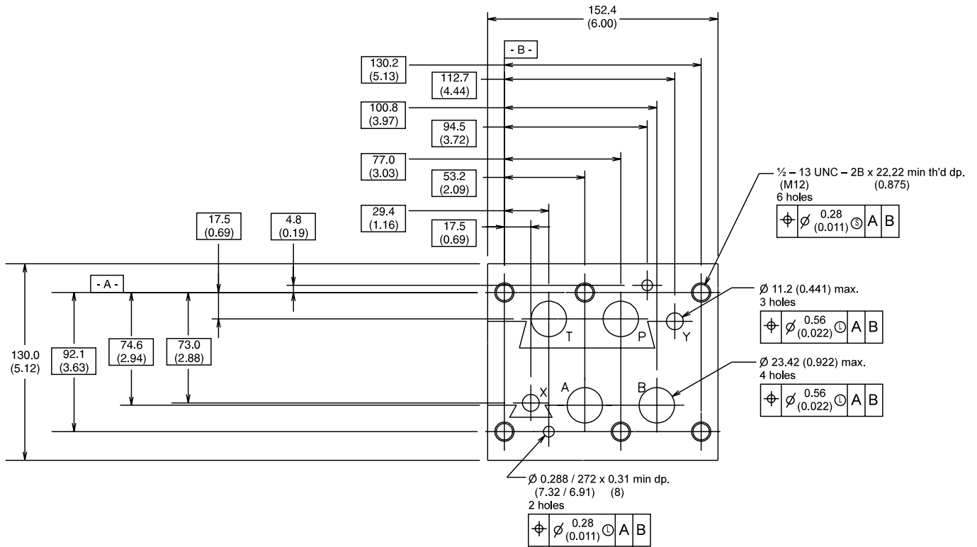
Mounting Surface for Directional Control Valve (NFFPA, D08); CETOP 8 & NG 25
