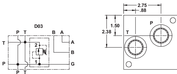
SPRP_03GSBSFUCA - BOTTOM VIEW
